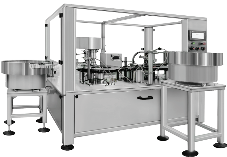
INHALER PACKING MACHINE
