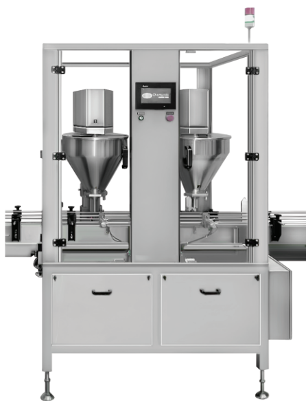
AUTOMATICS DOUBLE HEAD AUGER POWDER FILLING MACHINE
