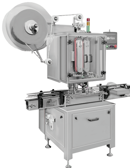
AUTOMATIC SILICA GEL POUCH / CANISTER INSERTER MACHINE
