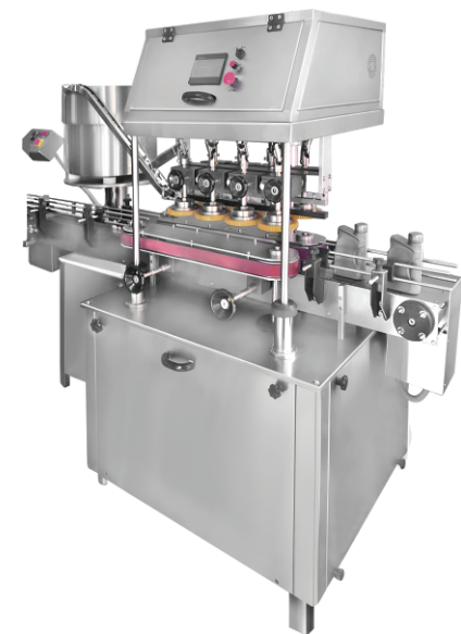
ONLINE SCREW CAPPING MACHINE WITH VIBRATOR BOWL
