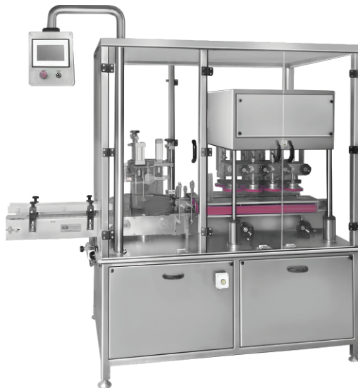
LINEAR TYPE INNER PLUG & SCREW CAPPING MACHINE
